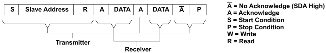
Figure 11. I 2 C Read Cycle
